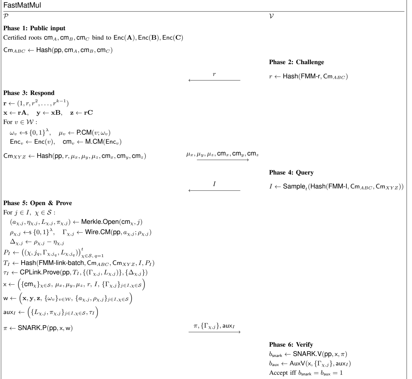
Figure 1. The FastMatMul protocol for verifiable matrix multiplication. \mathcal{S} = \mathcal{M} \cup \mathcal{W} is the set of objects opened at sampled positions, t = |I| is the query complexity, and \mathbf{x}, \mathbf{w} denote the public statement and witness for the inner SNARK.
