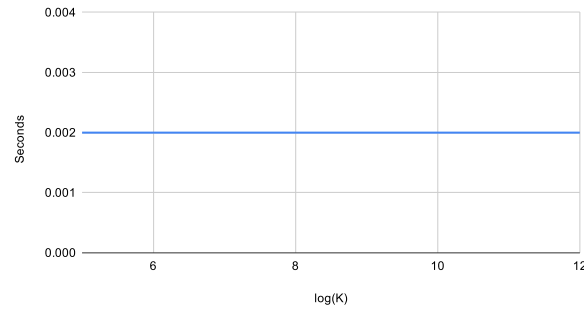
Verifying Time
