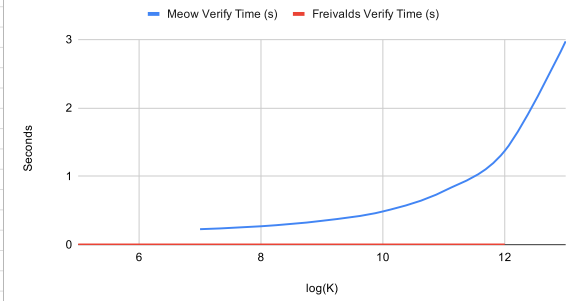
Verifying Time
