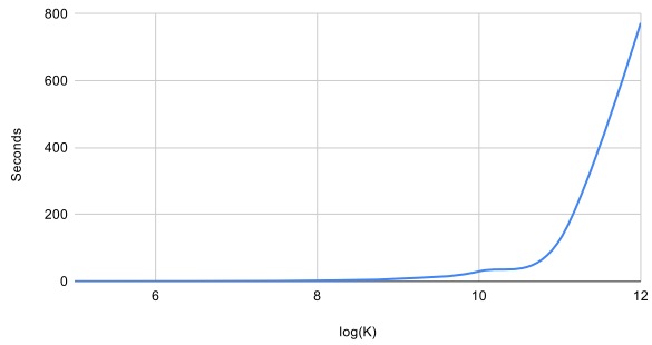
Proving Time
