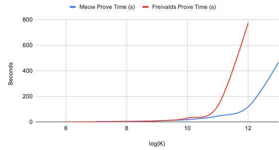
Proving Time
