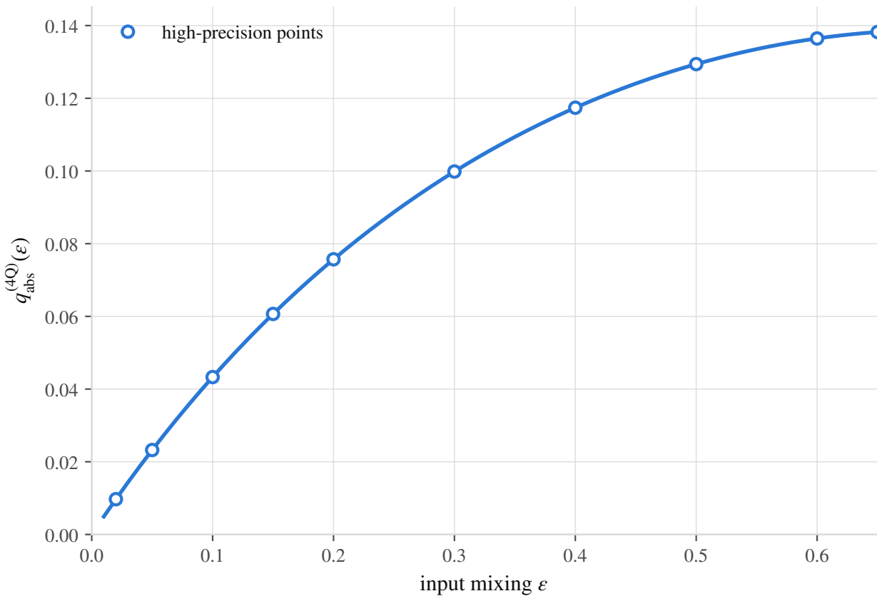
4Q: absolute Bell-error-suppression threshold (from the 5-CNOT postselected circuit simulation)
