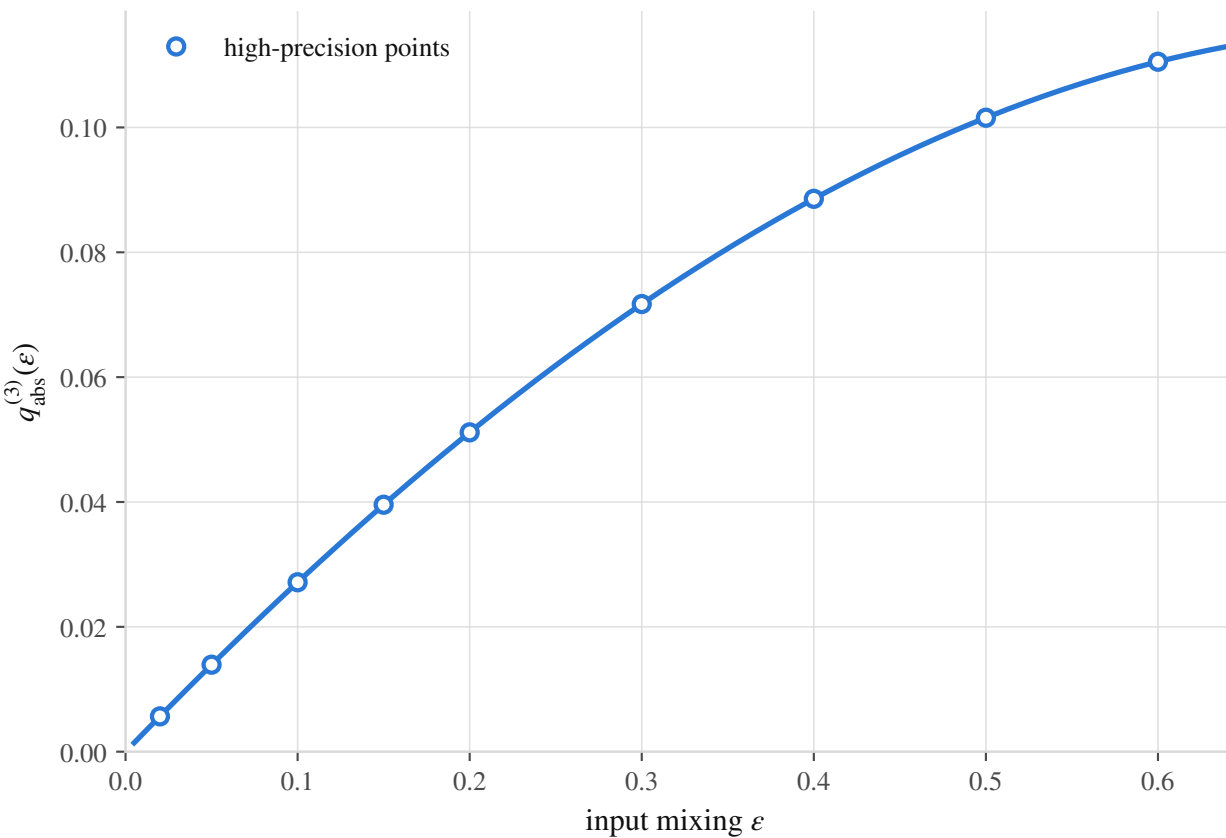
Type 3: absolute Bell-error-suppression threshold (from the 16-CNOT circuit simulation)
