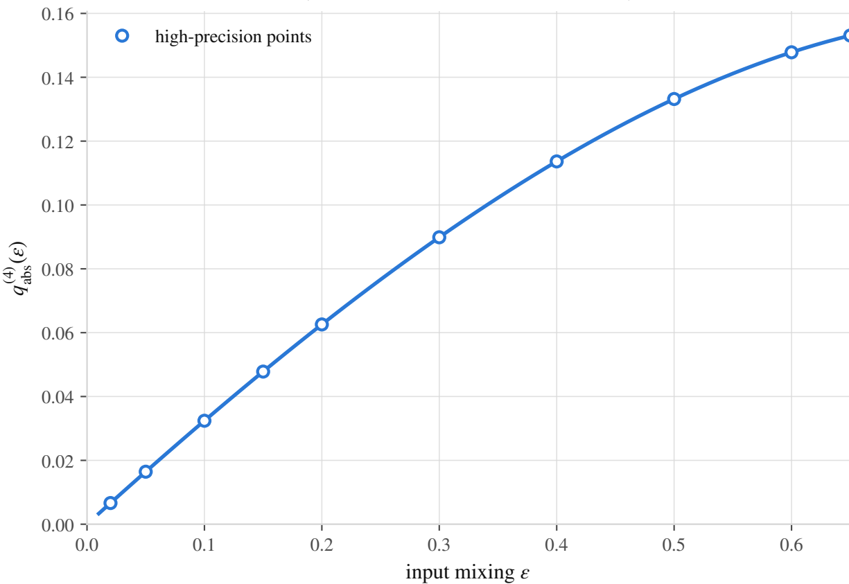
Type 4: absolute Bell-error-suppression threshold (from the 14-CNOT circuit simulation)
