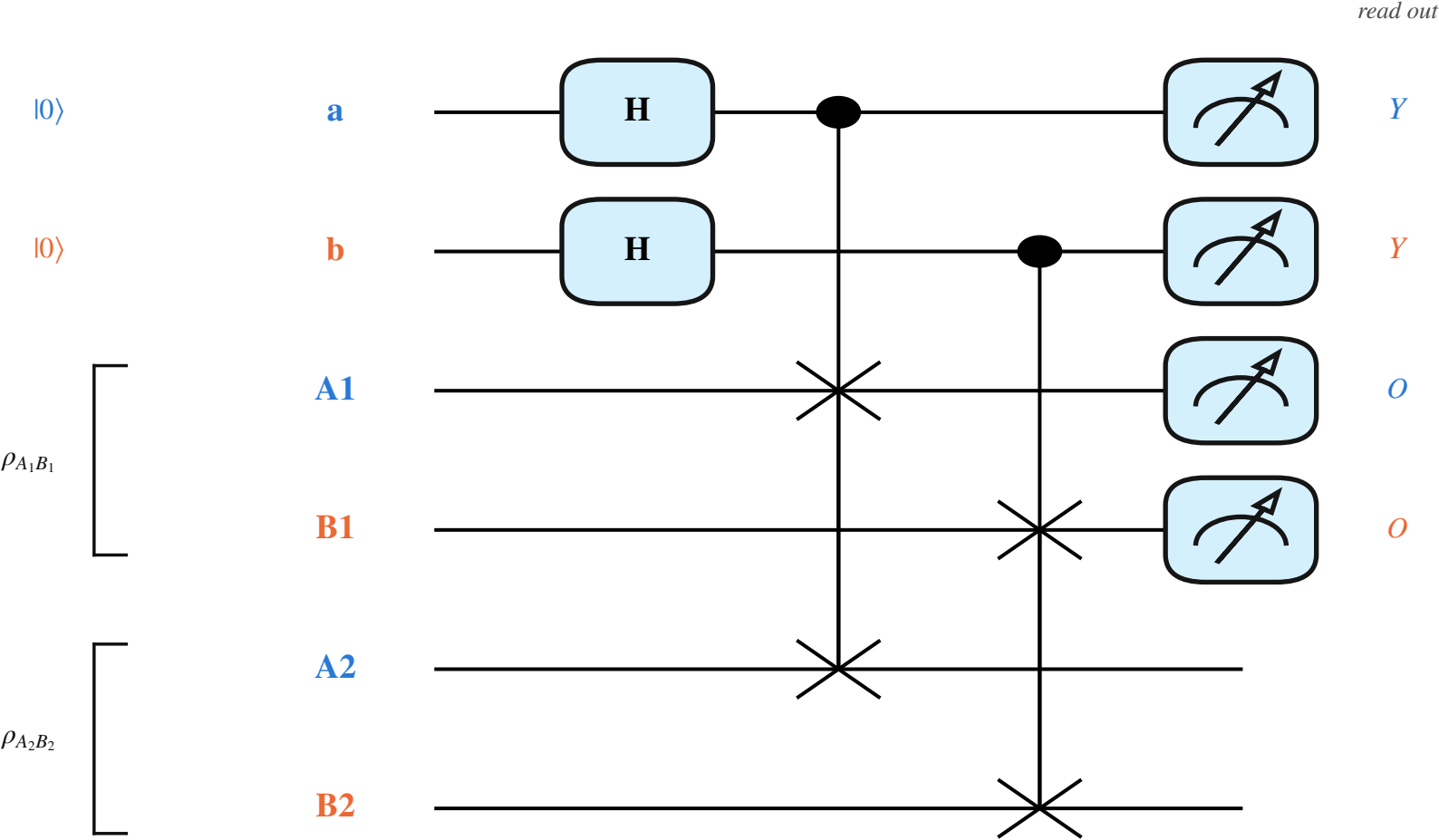
6Q LOCC SWAP-test circuit — \langle Y_a Y_b \otimes O_{A_1 B_1} \rangle (same gates, rotated read-out)
