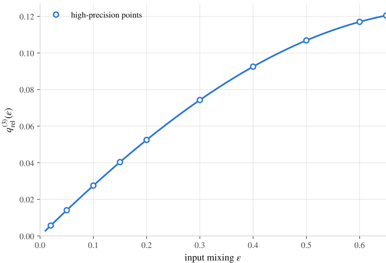
Type 3: relative Bell-error-suppression threshold (from the 16-CNOT circuit simulation)
