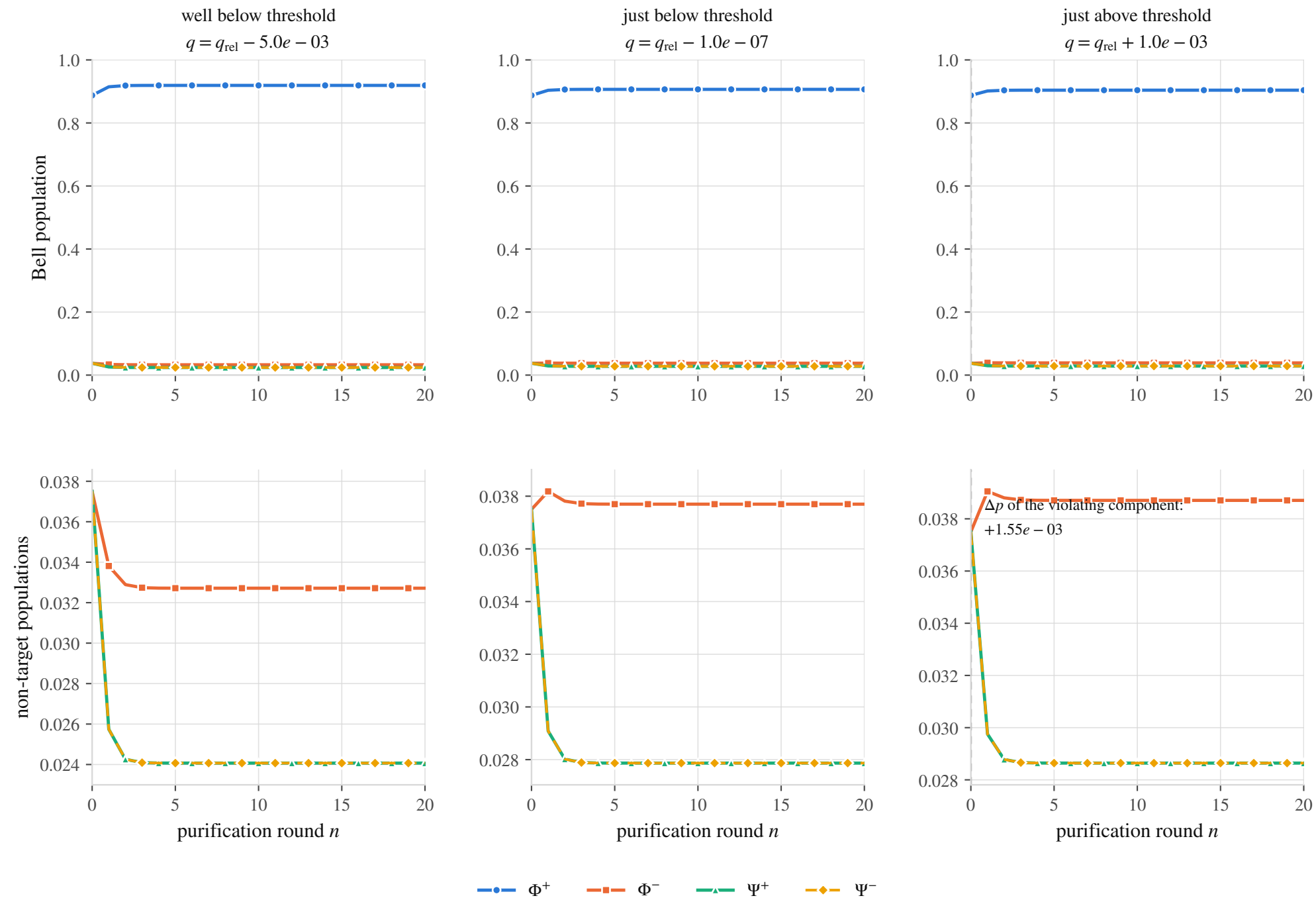
Type 3 at \varepsilon = 0.15 : raw Bell populations for the same three q
