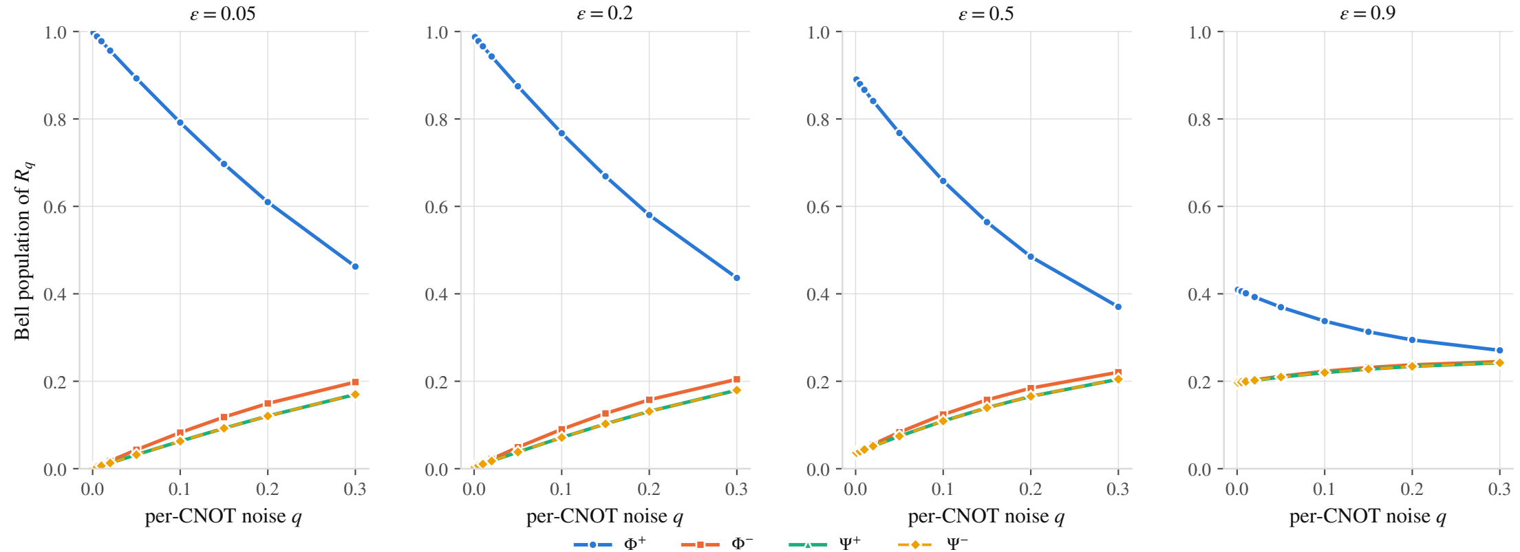
One noisy 6Q-L16 round: Bell populations of the reconstructed operator
