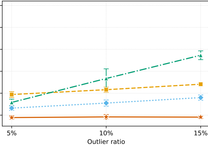
2D Allen-Cahn
