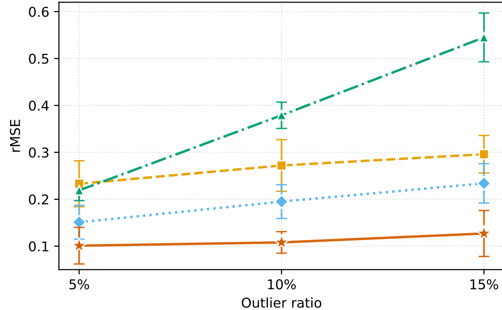
2D Burgers
