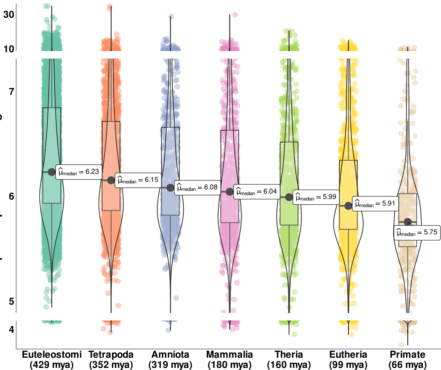
Gene pleiotropic scores for magnitude
