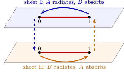
(a) \dot{n}_A = \mp \omega \sqrt{n_A n_B} : branch points n_A \in \{0, 1\} = S^0 , cut D^1
