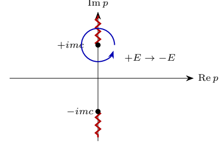
(b) E(p) = \sqrt{p^2 c^2 + m^2 c^4} : branch points at p = \pm imc
