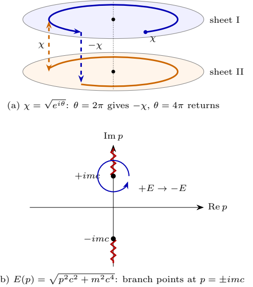
Fig. 11. The double cover as a Riemann surface
