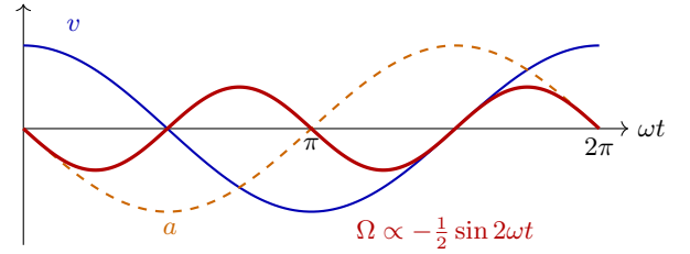
Fig. 13. Frequency doubling in the Thomas precession
