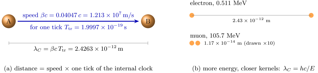
Fig. 15. Distance is made from the clock
