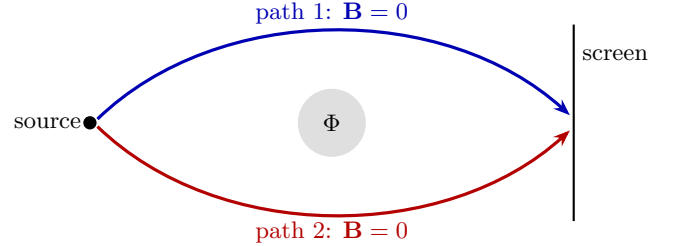
Fig. 17. Holonomy without a local field: the Aharonov–Bohm effect
