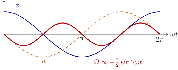
Fig. 13. Frequency doubling in the Thomas precession
