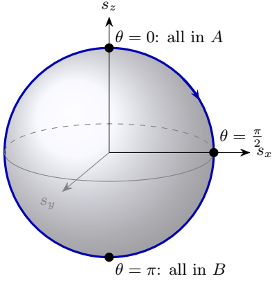
Fig. 11. The Bloch sphere and the electron's great circle
