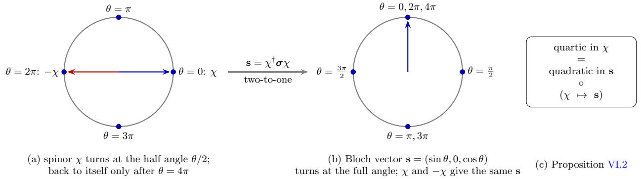
Fig. 12. The fourth power seen through the double cover
