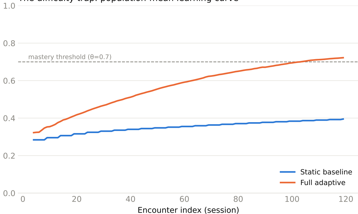
The difficulty trap: population-mean learning curve
