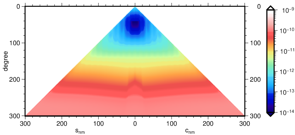
Figure 4.25: Formal errors of GOCO06s.
