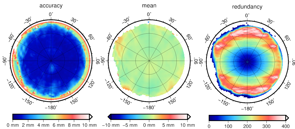
Figure 4.7: L2W accuracies of TerraSAR-X determined from residuals of one month
