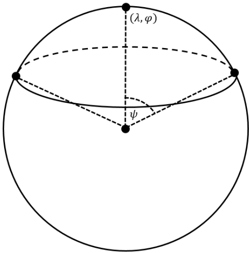
Figure 5.1: spherical cap
