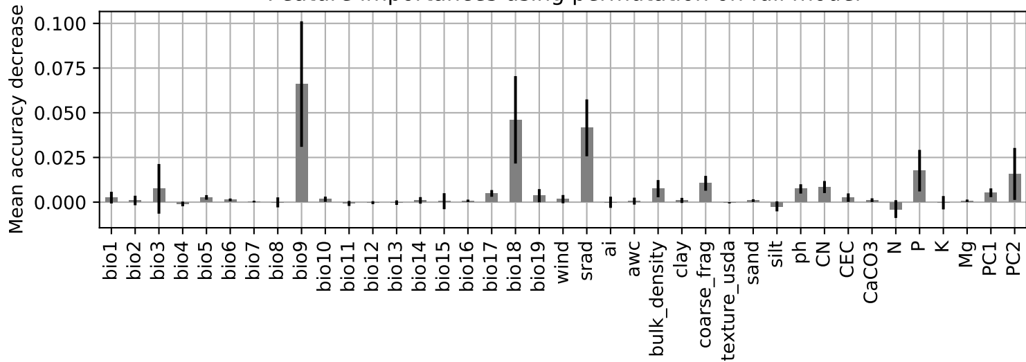
Feature importances using permutation on full model
