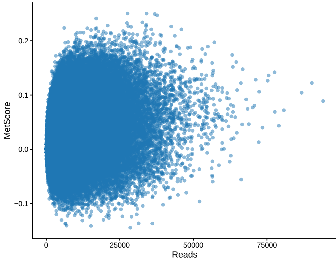
MetScore vs. Reads
