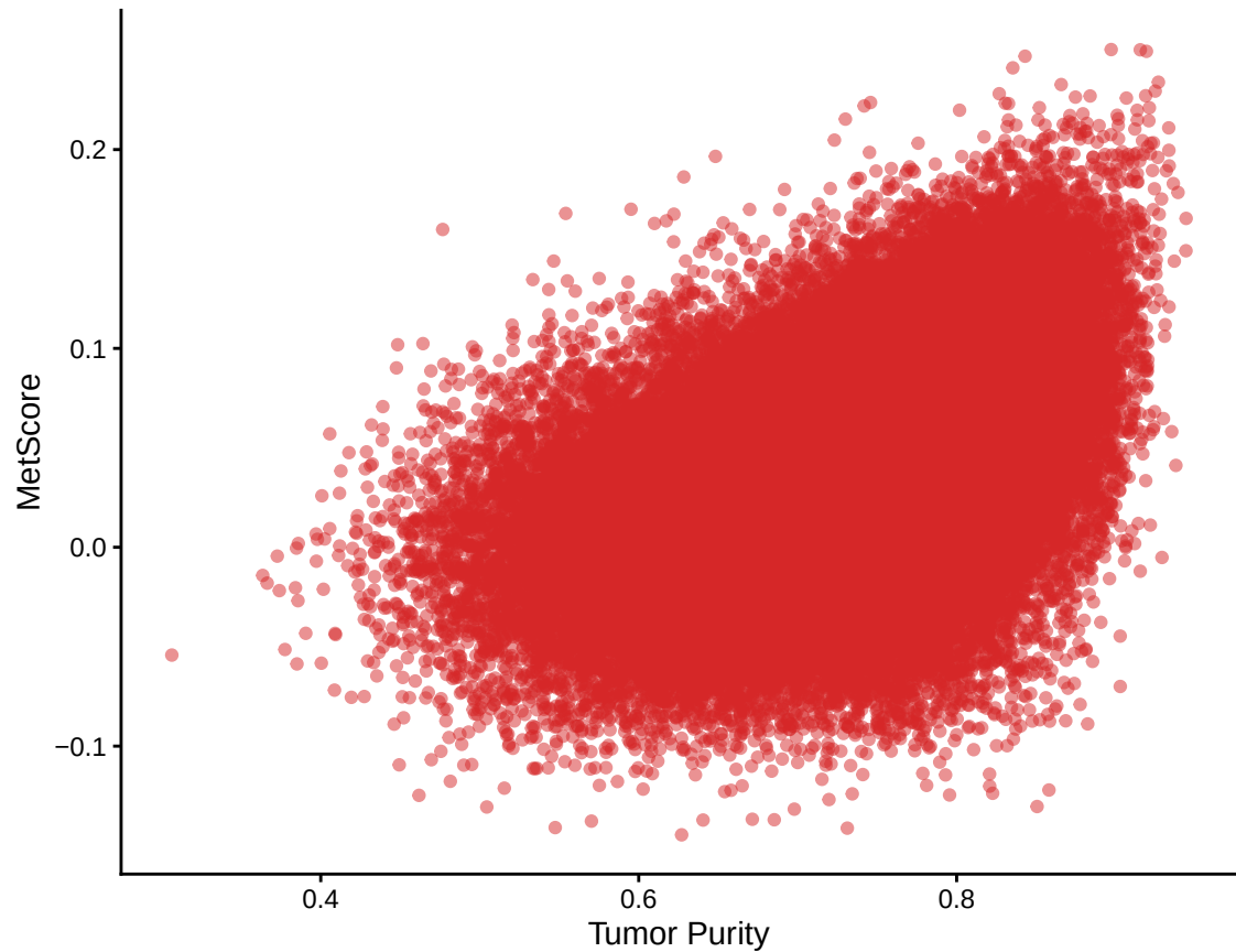
MetScore vs. Tumor Purity
