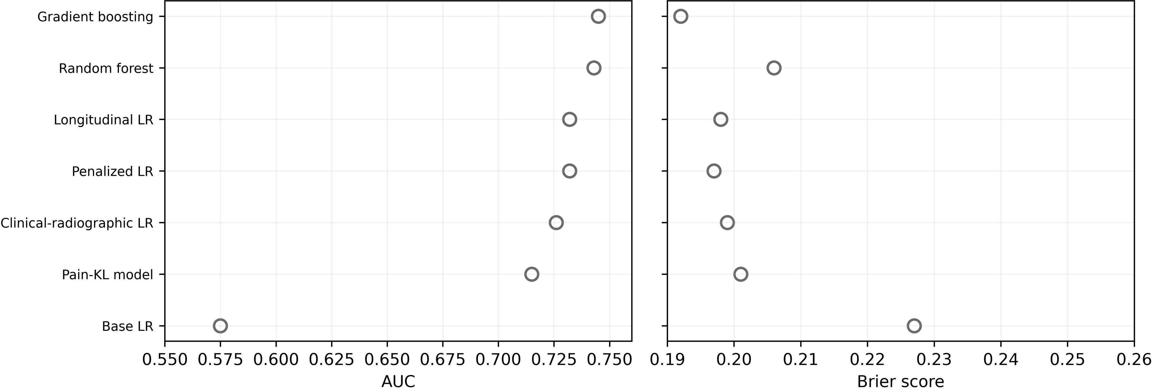
A. Discrimination
