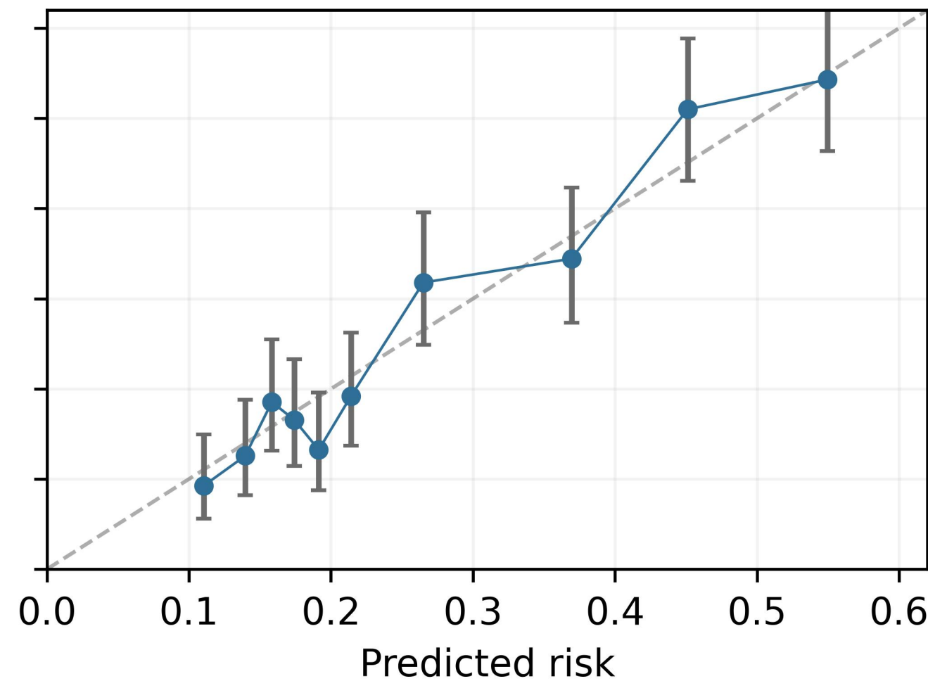
60-month: Penalized logistic regression
