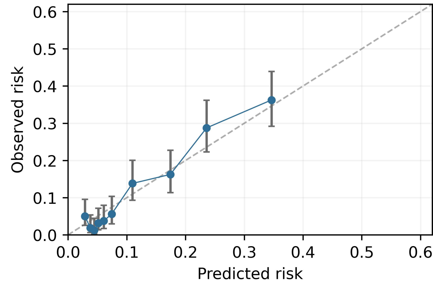
24-month: Penalized logistic regression
