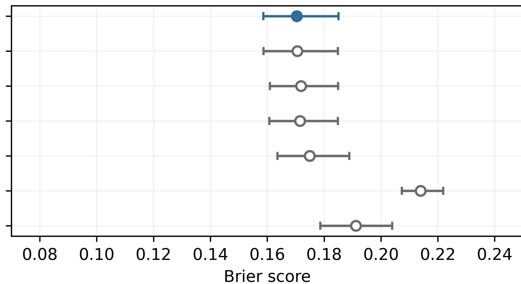
60-month Brier score (lower is better)
