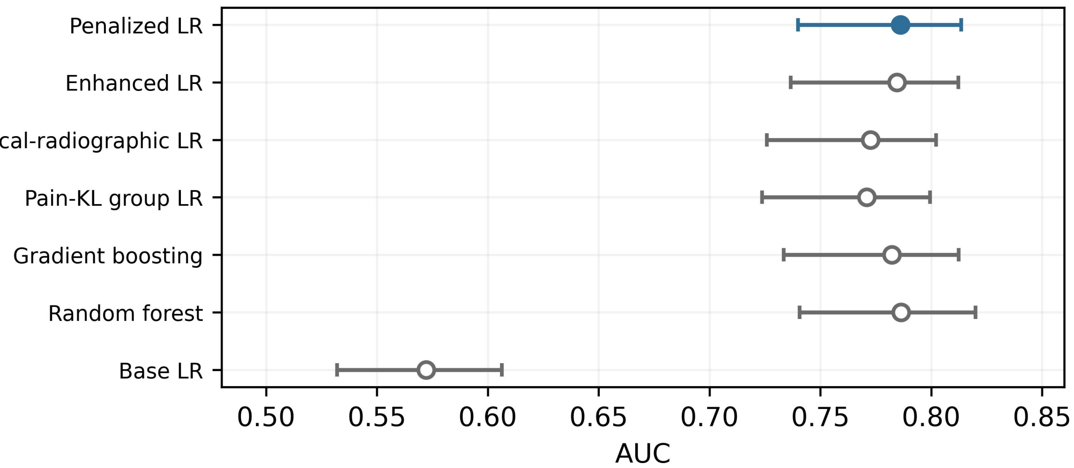
24-month AUC (higher is better)
