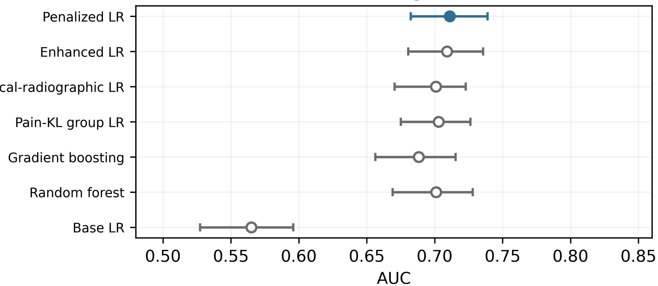
60-month AUC (higher is better)
