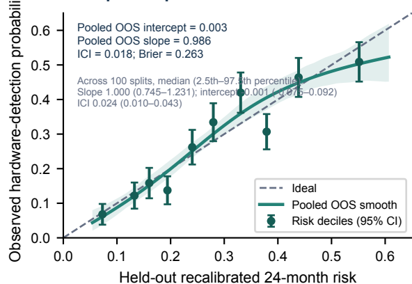
C. Repeated patient-level held-out recalibration
