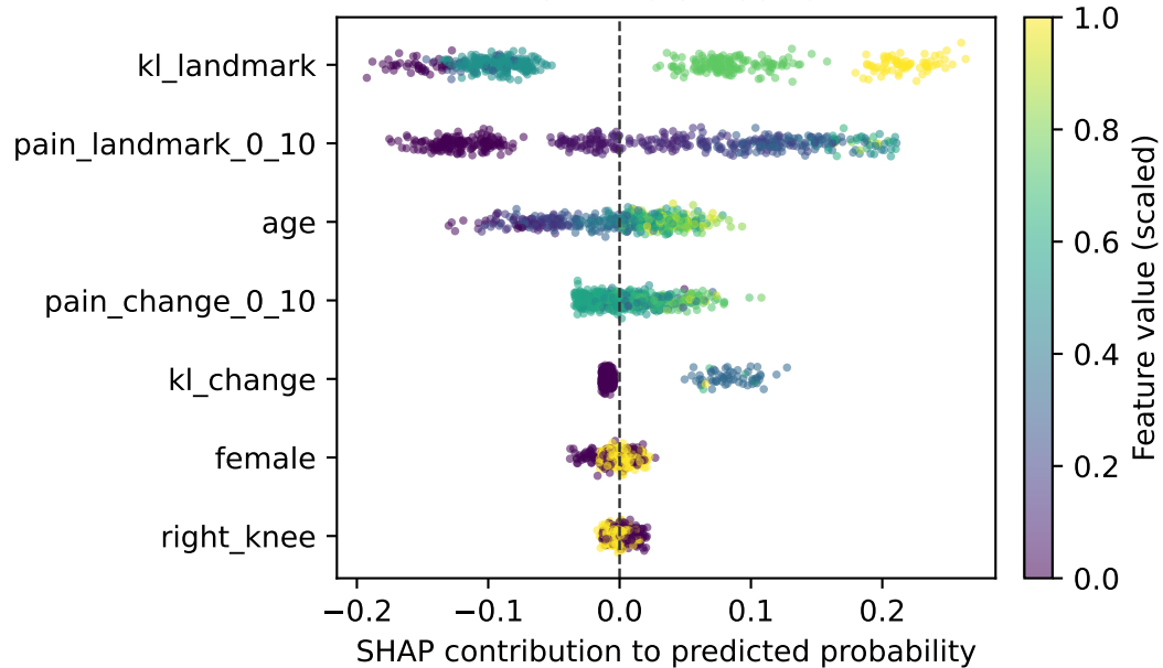
B. SHAP distribution
