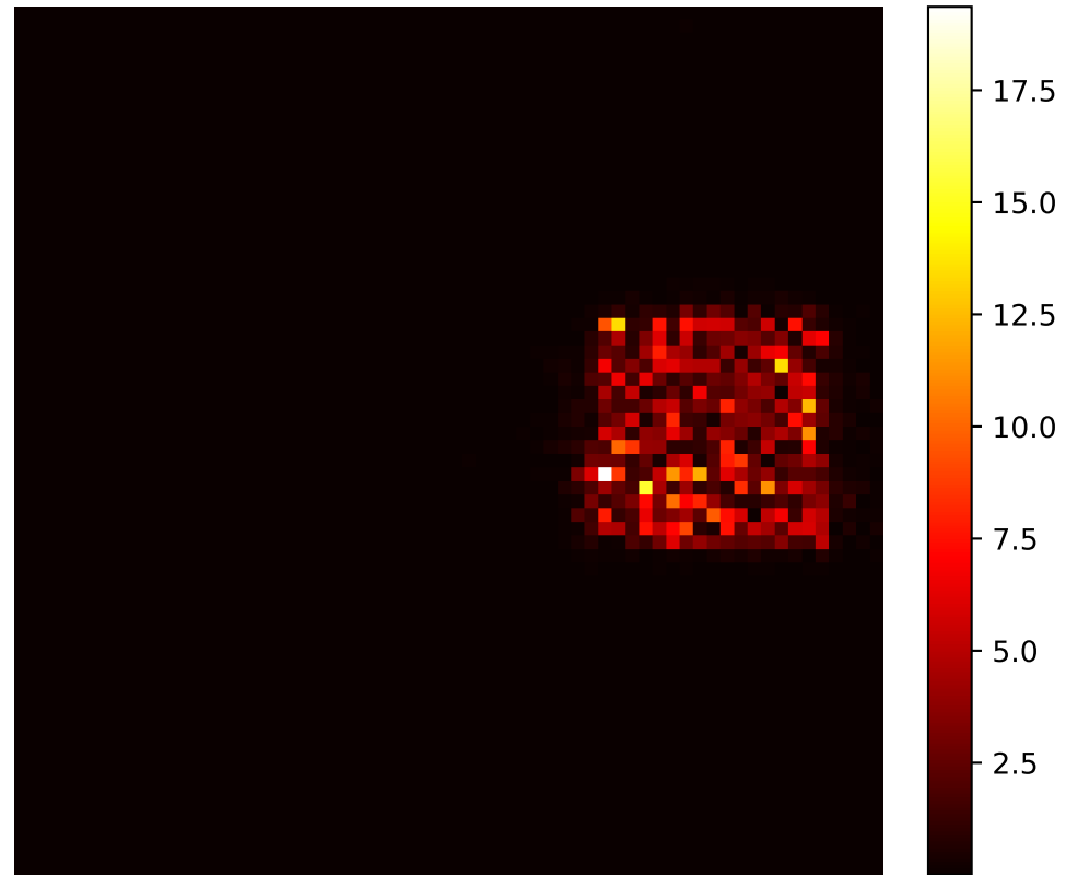
Inverse Energy Map ( x \rightarrow z'_T ) Sample ECR: 83.76% (Baseline: 6.25%)
