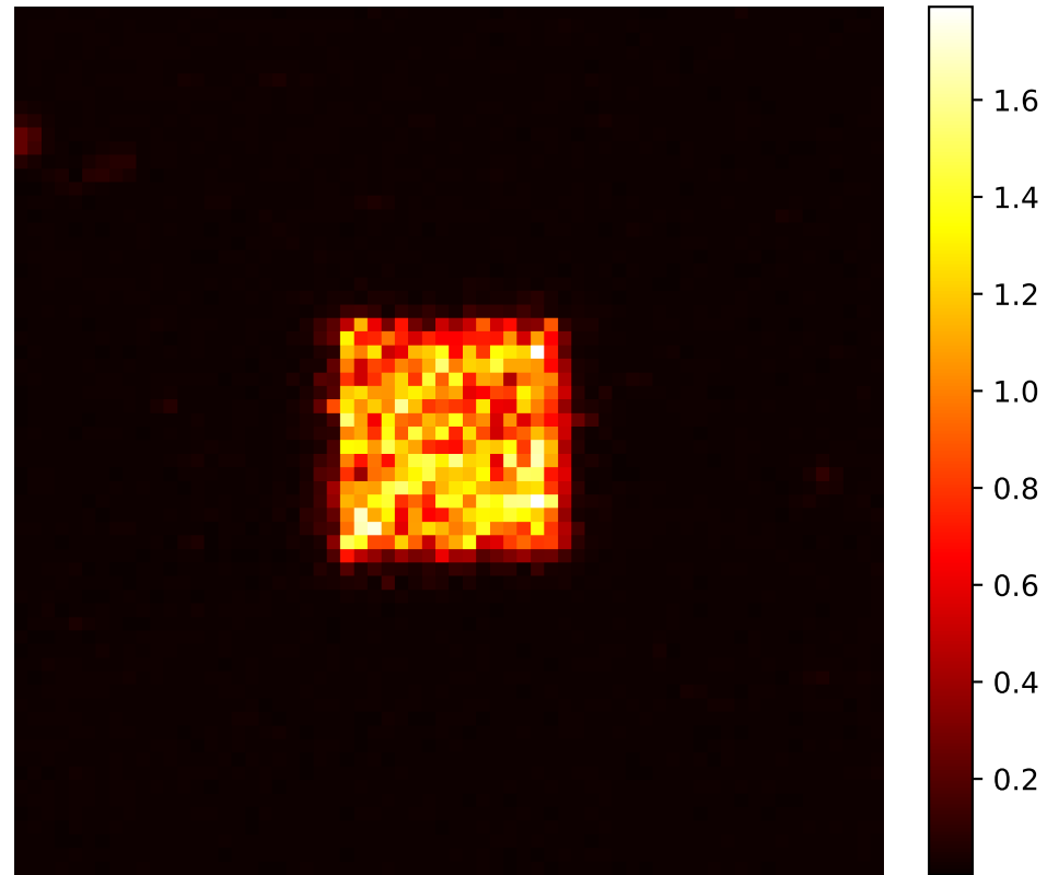
Inverse Mapping Diff ( x \rightarrow z'_T ) Center ECR: 95.31%
