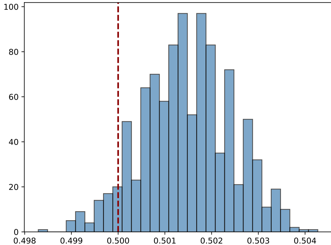
Empirical Distribution of \hat{p} (Ones Ratio)
