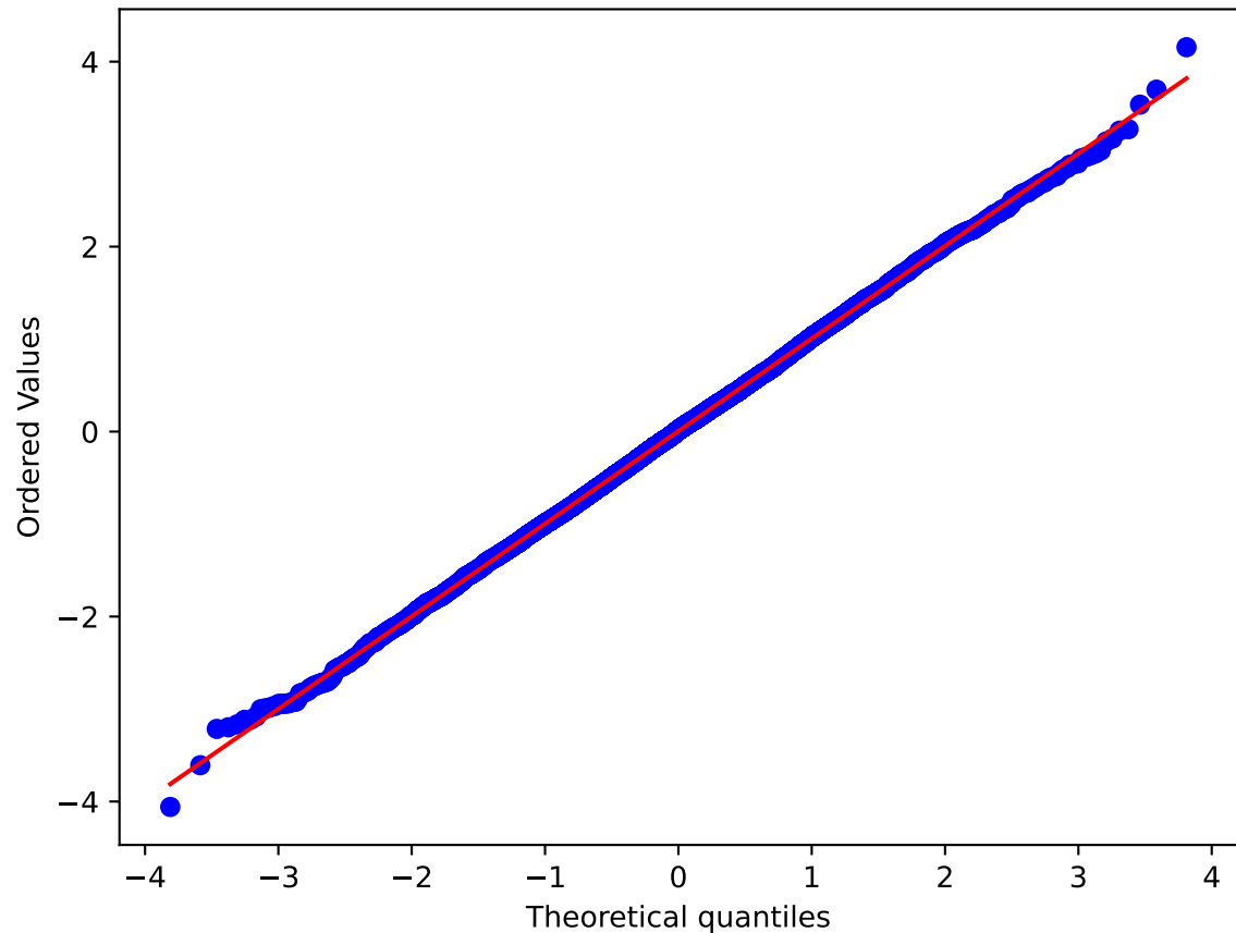
Q-Q Plot of Modulated Latents z_T
