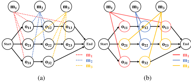
Fig. 4. Heterogeneous graph of the FJSP. Dotted line means processable, while solid line means scheduled. (a) Instance. (b) Solution.
