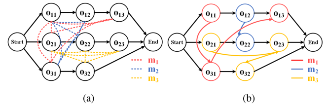
Fig. 2. Disjunctive graph of the FJSP. Dotted line means processable, while solid line means scheduled. (a) Instance. (b) Solution.
