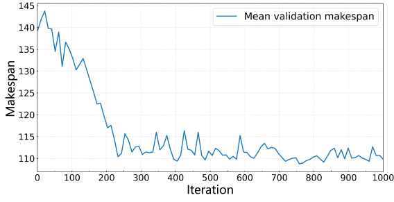
Fig. 7. Training curve on 10 \times 5 instances.
