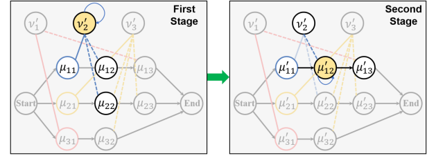
Fig. 5. Two-stage embedding scheme. Update of machine embedding \nu'_2 and operation embedding \mu'_{12} are highlighted for illustration.
