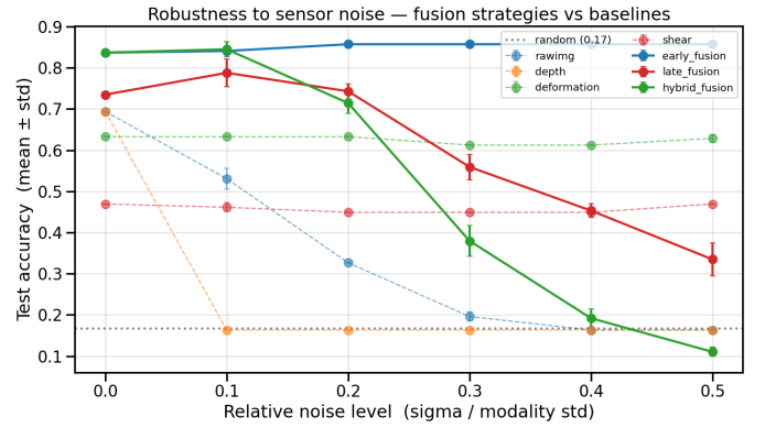
Fig. 3. Accuracy versus relative noise level (mean \pm std over five seeds). Early fusion (solid blue) is flat; hybrid fusion (solid green) starts tied with it then collapses below chance; late fusion (solid red) declines steadily.
