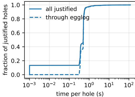
QF_UF
