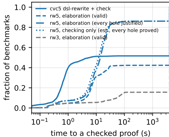
QF_UF (4316)
