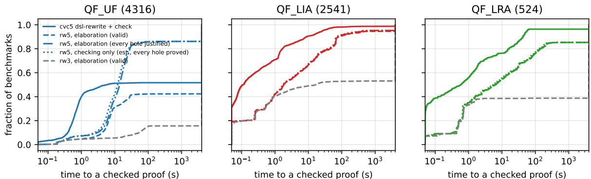
Figure 11: Time to a checked proof, as Figure 9 for rw5 ; grey dashed: rw3 with elaboration, proofs re-checked valid .
