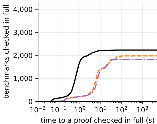
QF_UF (4,316 benchmarks)
