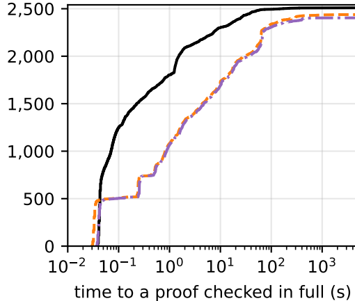
QF_LIA (2,541 benchmarks)
