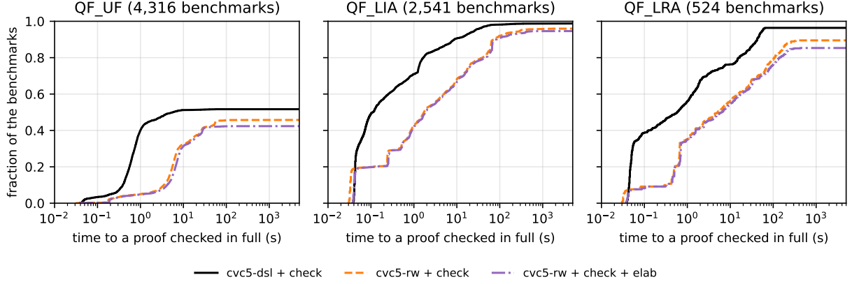
Figure 2: Time from benchmark to a proof checked in full, over every benchmark of each logic; a route’s line ends at the share of the benchmarks it checks in full. cvc5-dsl + check : cvc5 at dsl-rewrite and carcara check (dsl1) . cvc5-rw + check : cvc5 at rewrite , hoist and checking-only pass (estimated), every hole checked. cvc5-rw + check + elab : cvc5 at rewrite , hoist , elaboration pass and re-check (rw5) .
