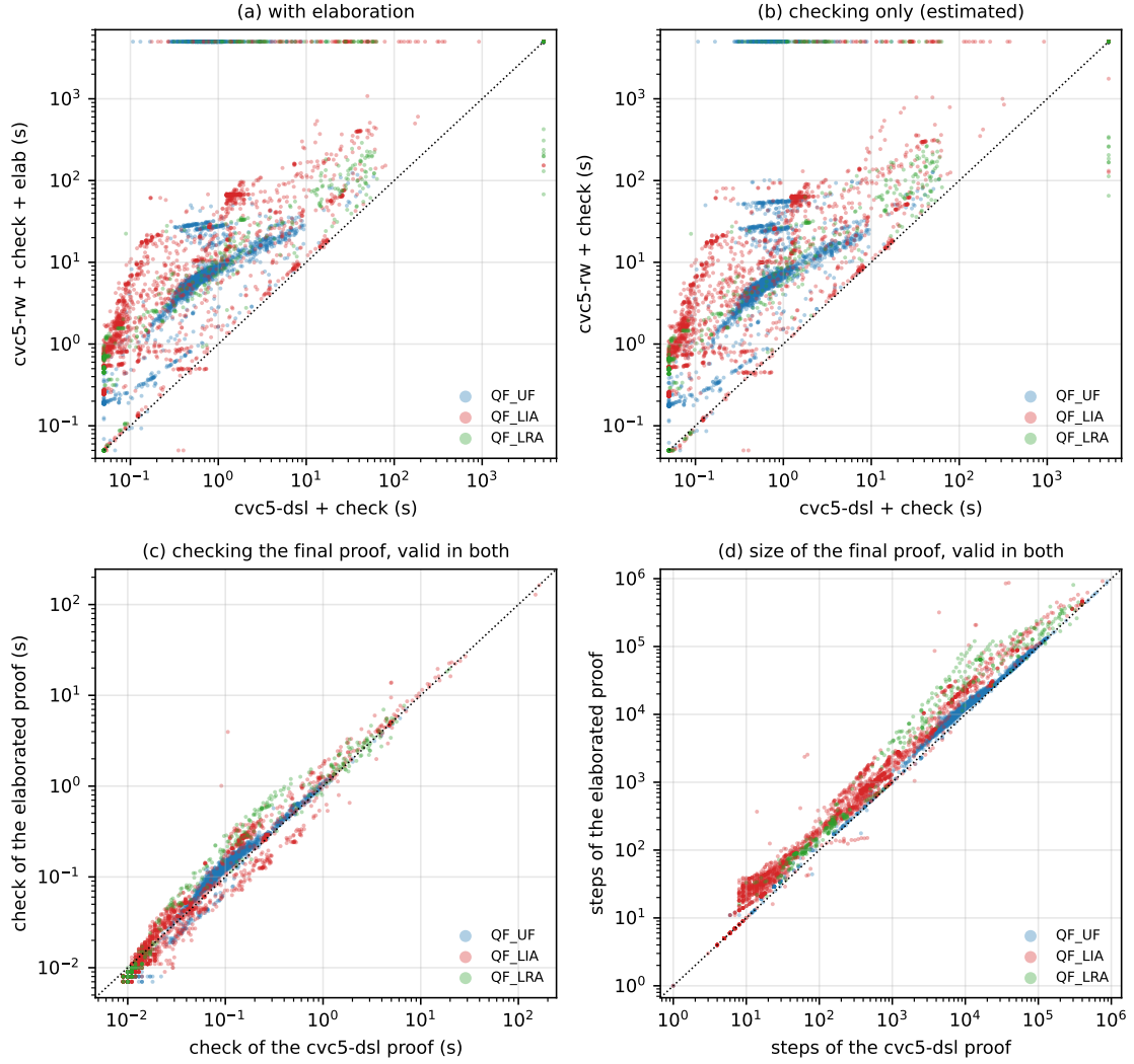
Figure 4: Per benchmark. (a), (b): cvc5-dsl + check ( x ) against cvc5-rw + check + elab and cvc5-rw + check ( y ), every benchmark; one a route does not check in full sits on that route's edge, one neither route checks in the corner. (c), (d): the 4,669 benchmarks valid in both, the check of the final proof and its number of steps, cvc5's own expansion ( x ) against the elaborated proof ( y ). The dotted line is y = x .
