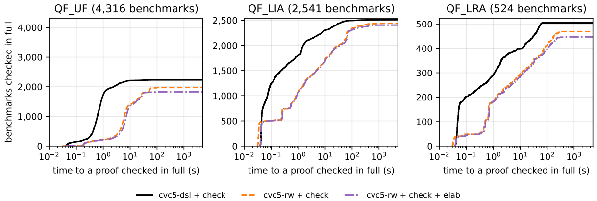
Figure 3: Figure 2 with the number of benchmarks on the y axis, each panel up to its logic’s number of benchmarks.
