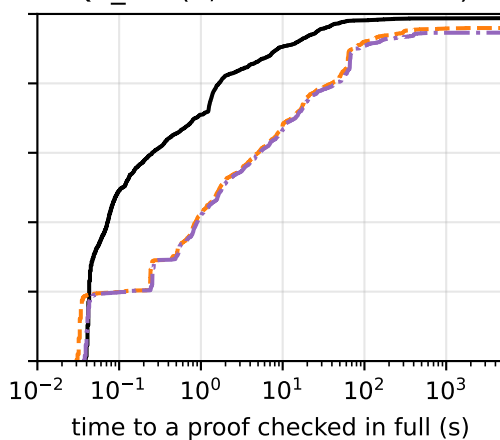
QF_LIA (2,541 benchmarks)
