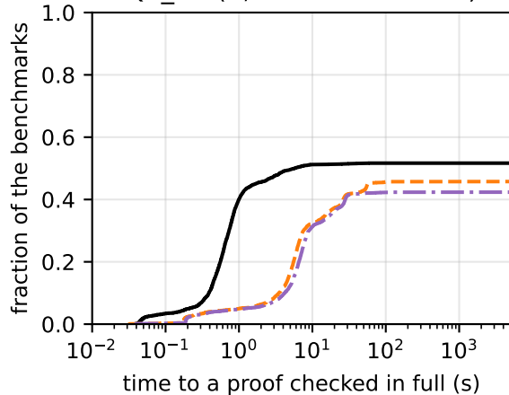
QF_UF (4,316 benchmarks)
