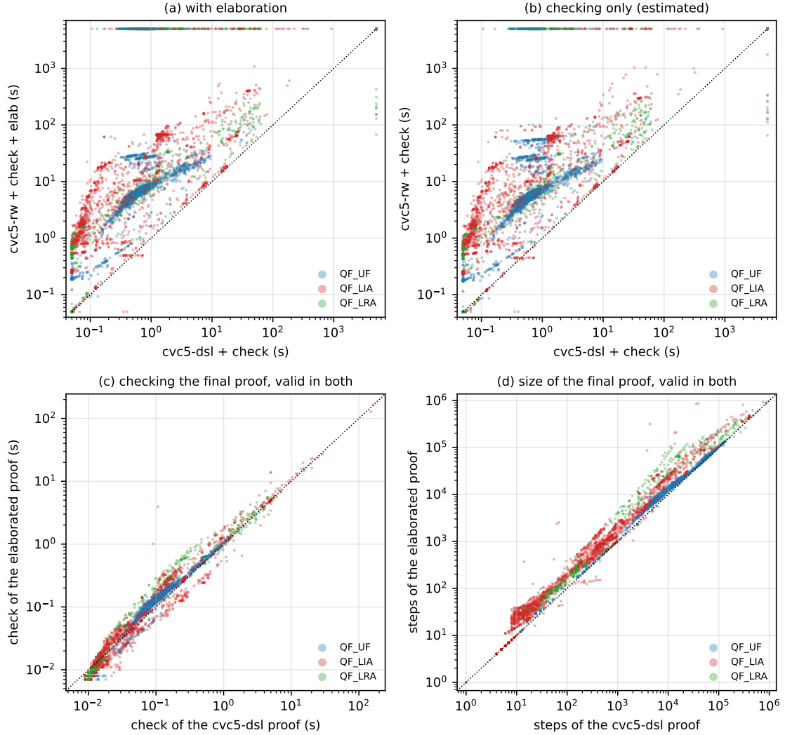
Figure 3: Per benchmark. (a), (b): cvc5-dsl + check ( x ) against cvc5-rw + check + elab and cvc5-rw + check ( y ), every benchmark; one a route does not check in full sits on that route's edge, one neither route checks in the corner. (c), (d): the 4,669 benchmarks valid in both, the check of the final proof and its number of steps, cvc5 's own expansion ( x ) against the elaborated proof ( y ). The dotted line is y = x .
