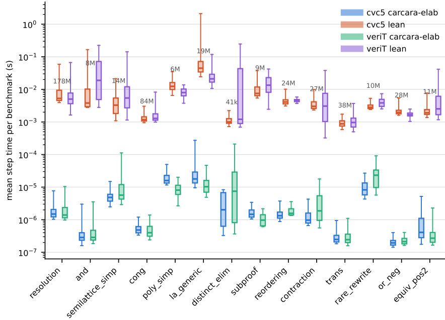
Fig. 4. Mean time per step of each rule, over the benchmarks whose elaborated proof both checkers accept, for the fourteen rules with the largest total time. Boxes are the quartiles and whiskers the 5th and 95th percentiles; the label above each group is the rule’s total step count in the round. Note the log scale: the two CARCARA series sit three to four decades below the two LEAN-SMT ones.
