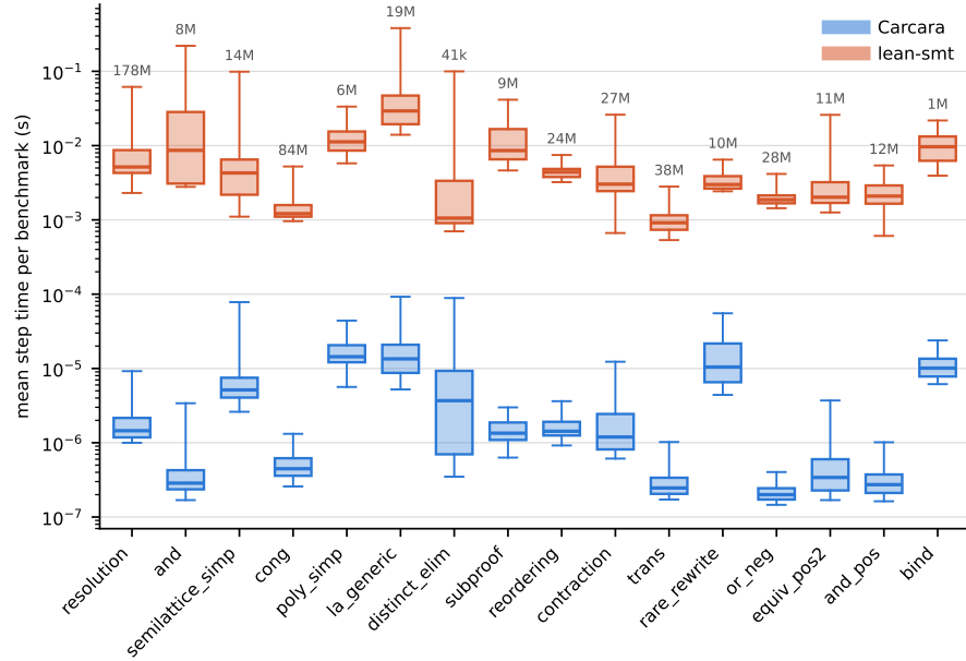
Fig. 4. Mean time per step of each rule, over the benchmarks whose elaborated proof both checkers accept, for the sixteen rules with the largest total time, pooling the two solvers. The two series share an x position. Boxes are the quartiles and whiskers the 5th and 95th percentiles; the label above each group is the rule’s total step count in the round. Note the log scale: CARCARA sits three to four decades below LEAN-SMT throughout.
