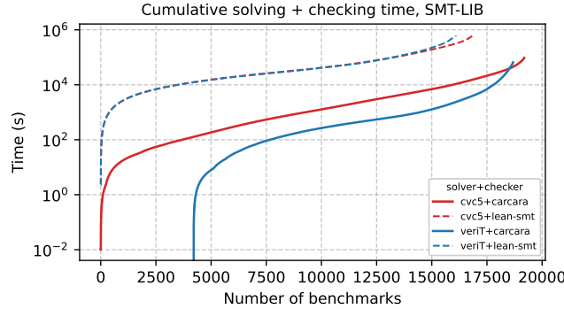
Fig. 3. Cumulative solving and checking time against the number of SMT-LIB benchmarks whose proof the configuration validated. CARCARA validates 19 188 CVC5 proofs in 26.6 CPU hours and 18 683 VERiT proofs in 18.1; the checker validates 16 912 and 16 098 in 184 and 171.
