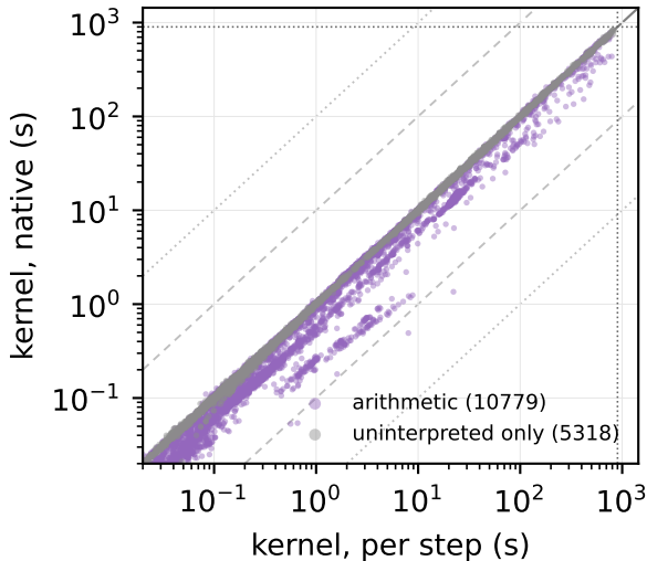
veriT, SMT-LIB: 16097 proofs
