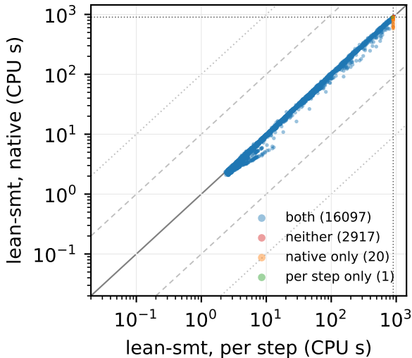
veriT, SMT-LIB: 19035 proofs
