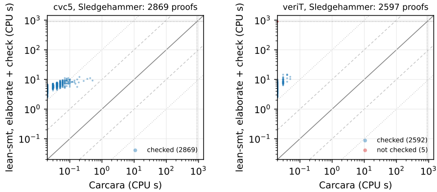
Fig. 5. CARCARA’s check against the elaboration plus LEAN-SMT’s check on the Sledgehammer proofs, CPU seconds. The band is the fixed cost of loading the library.
