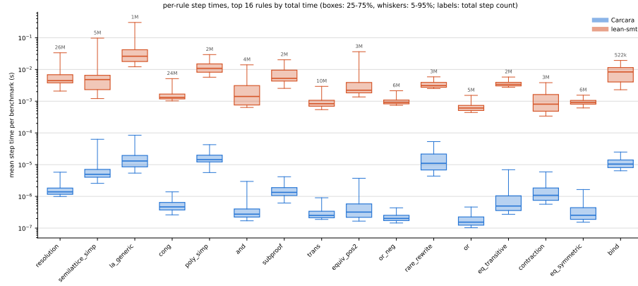
Fig. 4. Mean time per step of each rule, over the 18 153 benchmarks whose elaborated proof CARCARA accepts and the checker runs to the end, for the sixteen rules with the largest total time, pooling the two solvers. The two series share an x position. Boxes are the quartiles and whiskers the 5th and 95th percentiles; the label above each group is the rule’s step count over that population, which is the same number for both tools — they are counting the steps of the same proofs. Note the log scale: CARCARA sits three to four decades below LEAN-SMT throughout.
