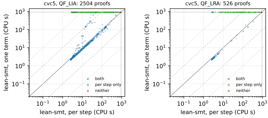
Fig. 8. The same comparison on cvc5’s arithmetic proofs, QF_LIA (left) and QF_LRA (right). The proofs are smaller, so both shapes reach further, and the one-term shape still loses 812 and 217 benchmarks.
