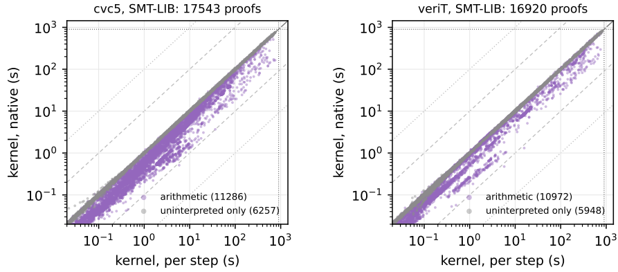
Fig. 11. The kernel’s own time in the two arms, on the proofs both validate, seconds; the proofs of a logic with arithmetic are drawn apart from those of QF_UF and UF. The saving is where the normalizer runs: the uninterpreted proofs lie on the diagonal, the arithmetic ones below it.
