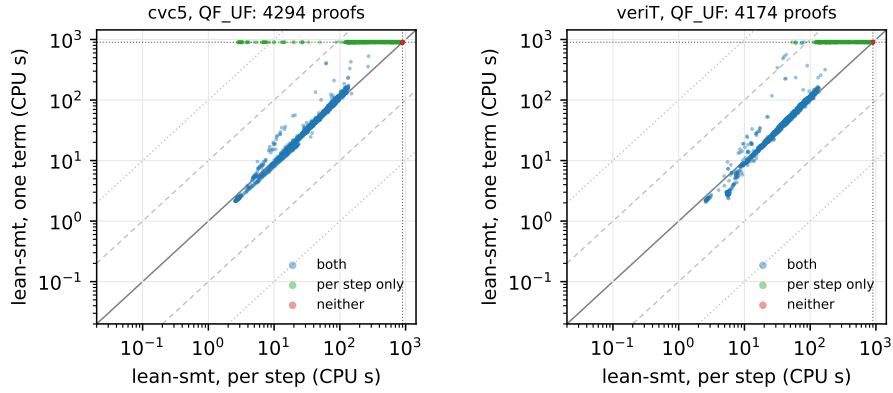
Fig. 7. The two kernel submission shapes on the same QF_UF proofs, CPU seconds. A point on a dotted border is a proof the corresponding shape did not check; the grey lines are equality and factors of ten and a hundred.
