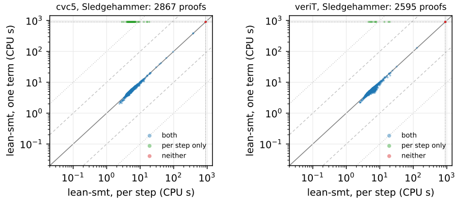
Fig. 9. The two submission shapes on the Sledgehammer proofs, CPU seconds. The band along the diagonal is the fixed cost of loading the library.
