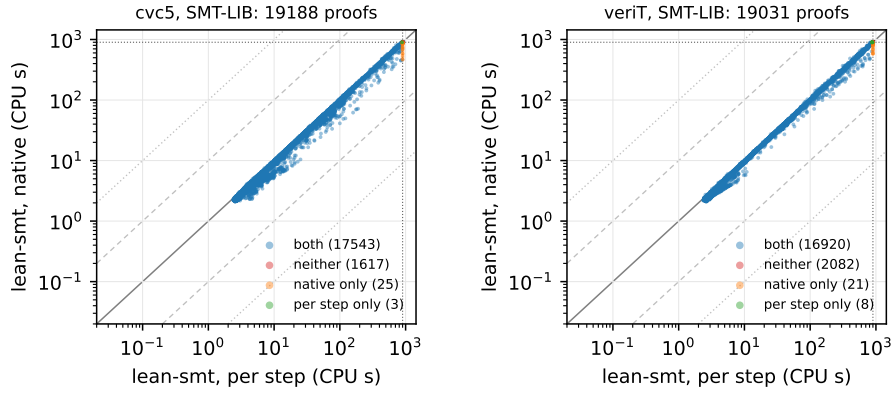
Fig. 10. The per-step shape against its native variant on the same SMT-LIB proofs, CPU seconds. A point on a dotted border is a proof the corresponding arm did not validate; the grey lines are equality and factors of ten and a hundred. The cloud sits just below the diagonal, and the points either arm loses alone are all against the limit.
