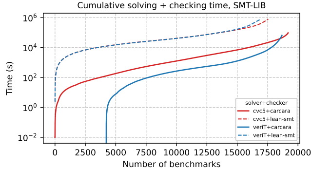
Fig. 3. Cumulative solving and checking time against the number of SMT-LIB benchmarks whose proof the configuration validated. CARCARA validates 19 188 CVC5 proofs in 26.8 CPU hours and 18 680 VERiT proofs in 18.1; the checker validates 17 546 and 16 928 in 219 and 223.
