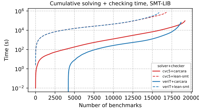
Fig. 3. Cumulative solving and checking time against the number of SMT-LIB benchmarks whose proof the configuration validated. CARCARA validates 19 190 CVC5 proofs in 26.7 CPU hours and 18 688 VERiT proofs in 18.5; the checker validates 16 813 and 15 870 in 206 and 192.
