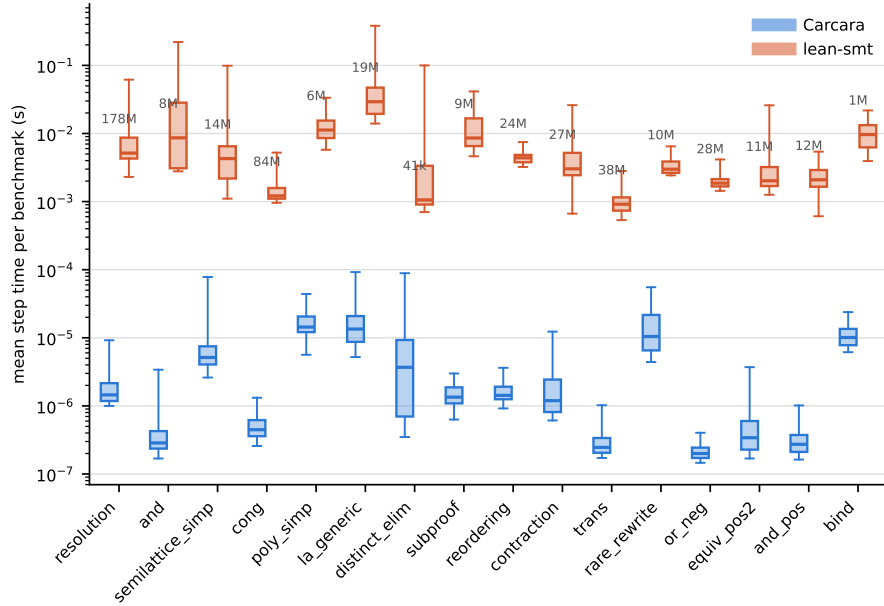
Fig. 4. Mean time per step of each rule, over the benchmarks whose elaborated proof both checkers accept, for the sixteen rules with the largest total time, pooling the two solvers. Boxes are the quartiles and whiskers the 5th and 95th percentiles; the label above each group is the rule’s total step count in the round. Note the log scale: CARCARA sits three to four decades below LEAN-SMT throughout.
