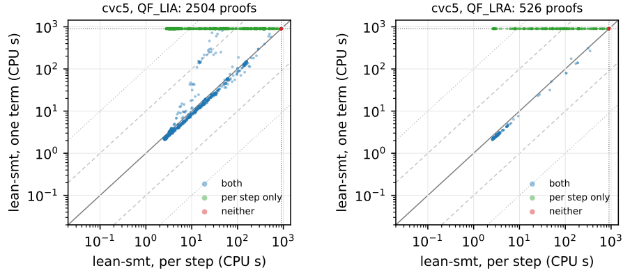
Fig. 8. The same comparison on cvc5 's arithmetic proofs, QF_LIA (left) and QF_LRA (right). The proofs are smaller, so both shapes reach further, and the one-term shape still loses 812 and 217 benchmarks.
