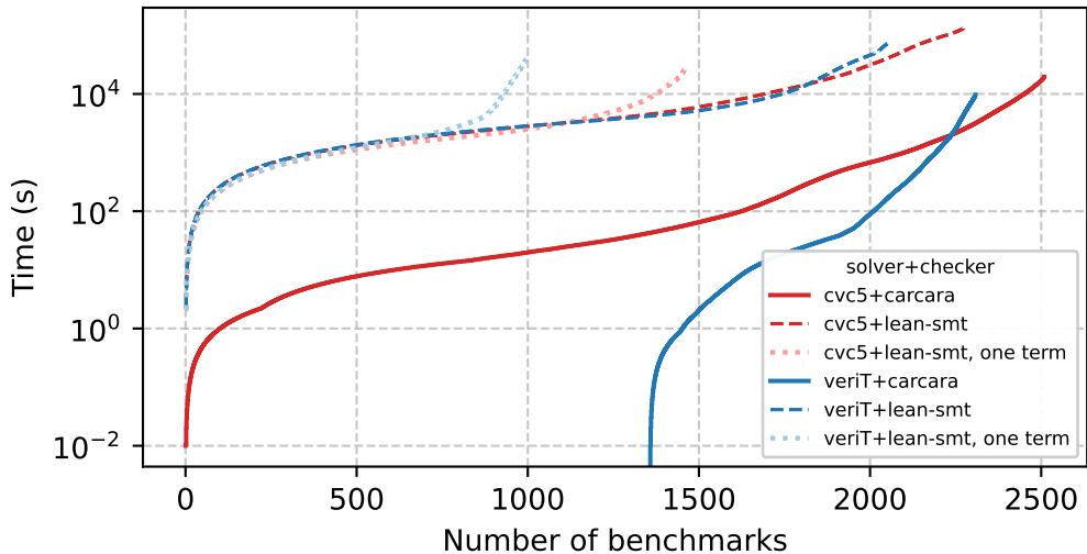
Cumulative solving + checking time, QF_LIA
