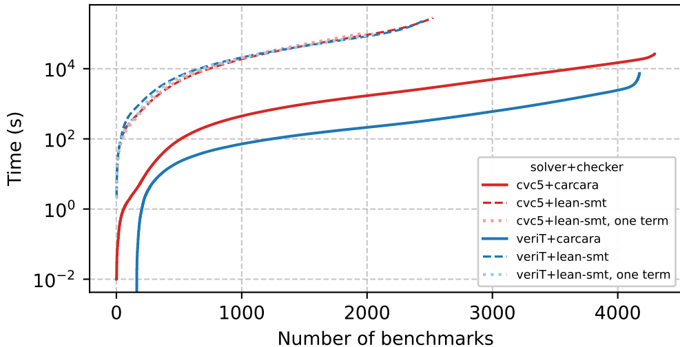
Cumulative solving + checking time, QF_UF
