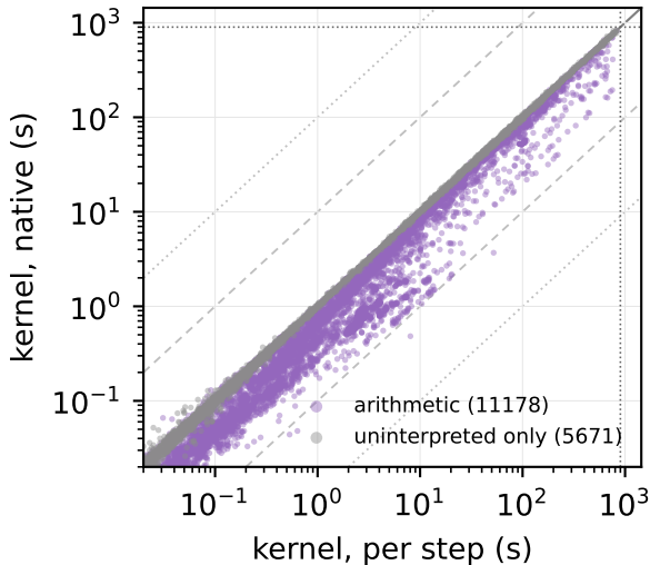
cvc5, SMT-LIB: 16849 proofs
