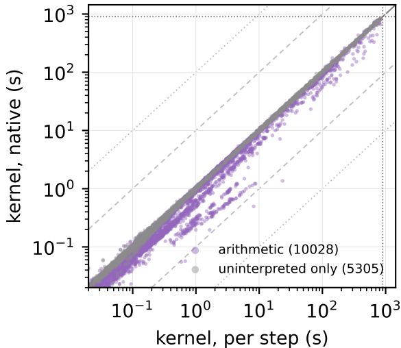
veriT, SMT-LIB: 15333 proofs
