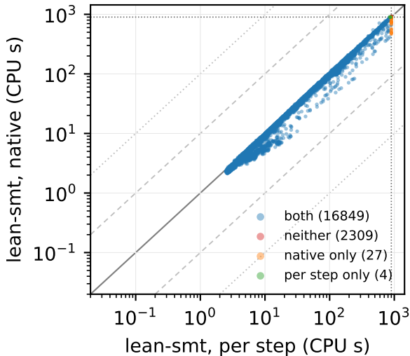
cvc5, SMT-LIB: 19189 proofs
